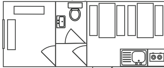
20'x8' Canteen/Drying Room/Toilet with Gas Handwash
