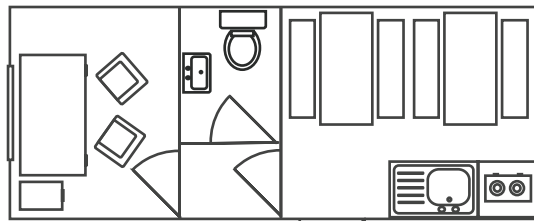
20'x8' Office/Canteen/Toilet with Gas Handwash
